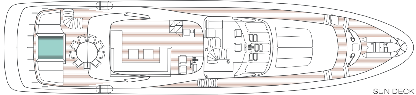
SUN DECK
