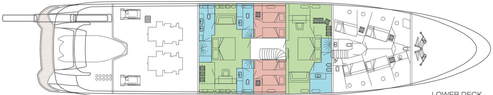
LOWER DECK
